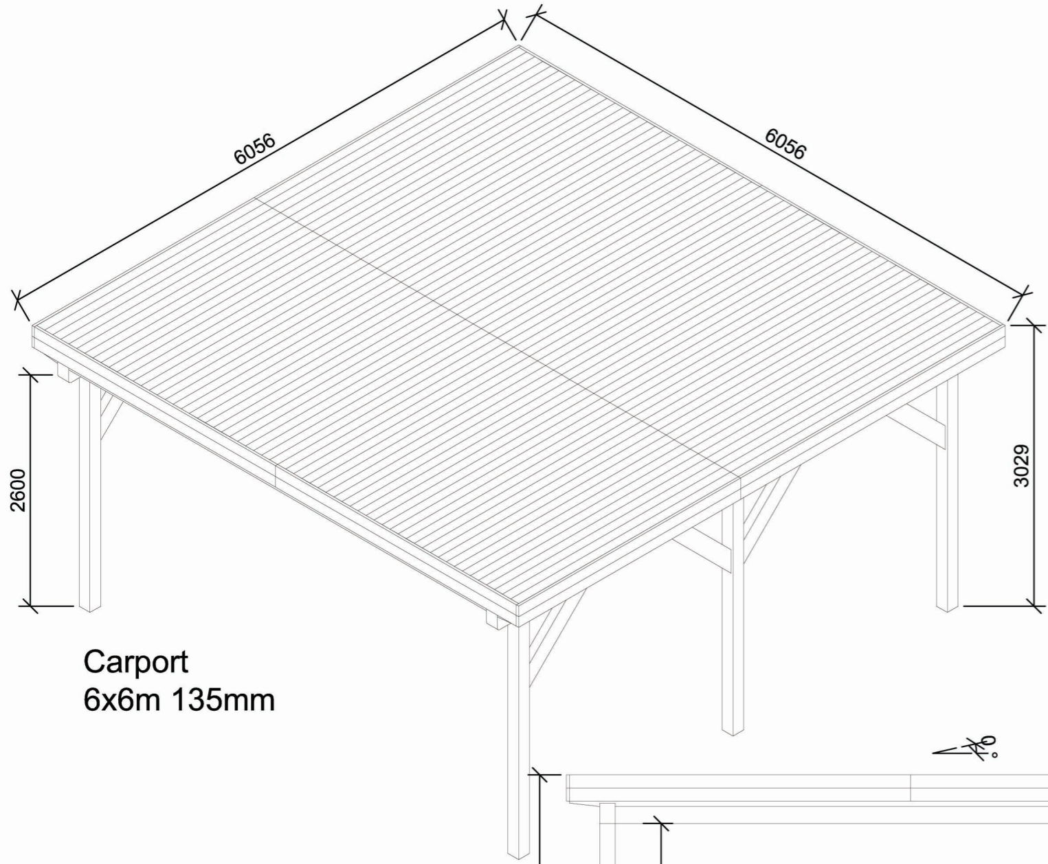
Carport 6x6m 135mm
