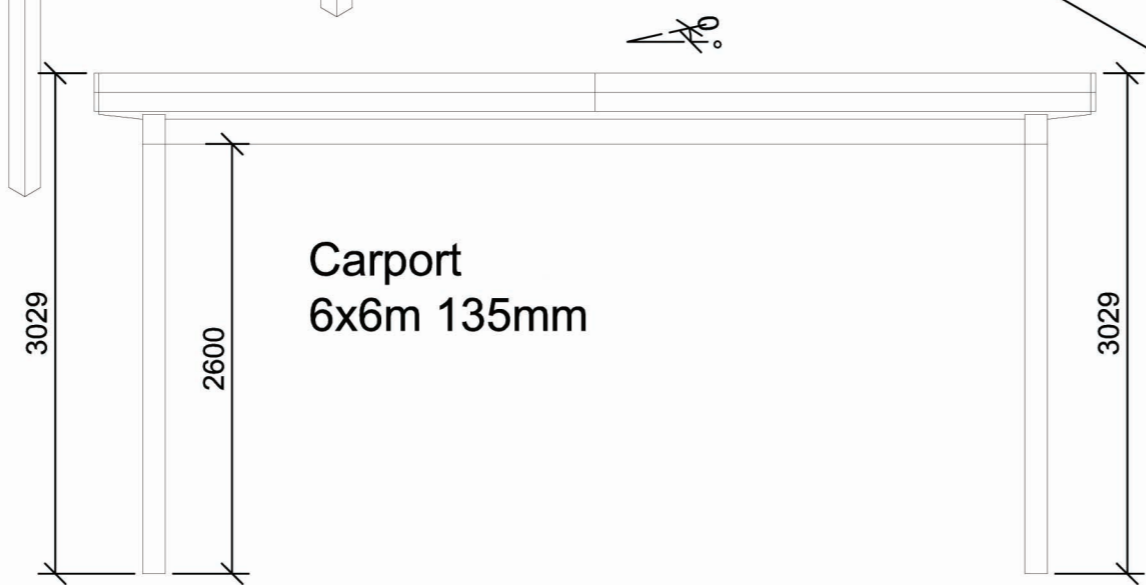
Carport 6x6m 135mm
